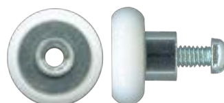
3-4290 Roller • Suit shower door 19mm. Hub: 6mm. Load: 8kg. Threaded hub. Acetal convex roller with bearing. Suits Boral Elite. Use with 2-7010 bracket.
