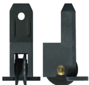
3-5141 Carriage adjustable & roller Suit window Acetal concave roller and brass axle pin. 12kg. Adjustable vertically. Suits old Bradnams.
