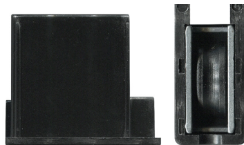
3-1208 Carriage adjustable & roller Suit patio door Suits Southern Star. 25kg. Acetal roller with bearing.
