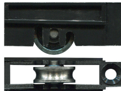
3-5111 Carriage adjustable & roller Suit window Three adjustment heights. 12kg. Stainless steel concave roller and bearing. Suits GJames and others. Can use 3-4191 as replacement roller. Nylon version is 3-5011.
