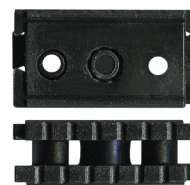
3-5200 Carriage & roller Suit window Multi-link. 15kg. Black. Acetal flat roller and plastic axle pin. Replaces old model. Can use 3-5201. Suits Boral BST.
