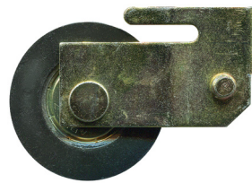
3-1061 Carriage & roller Suit patio door Use with 3-1051 bracket. 25kg. Acetal roller with bearing. Suits Boral KM Cyclone, GJames and some wardrobes.
