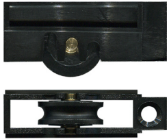
3-5011 Carriage adjustable & roller Suit window Three adjustment heights. 8kg. Acetal concave roller and brass axle pin. Suits Alcan and GJames School Suite. For heavier duty (12kg), use 3-4190 as a replacement roller, or use 3-5111.
