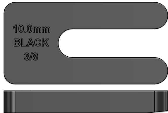
4-0100 10.0mm door and window packer – Black.
