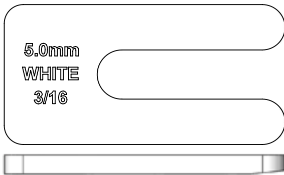
4-0050 5.0mm door & window packer – White.
